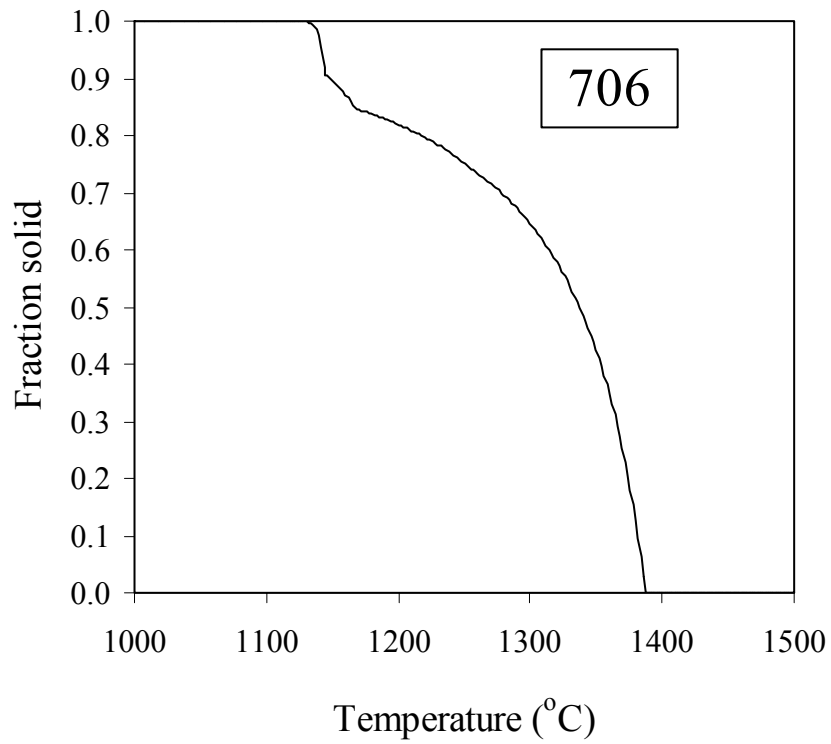
Figure 2. Calculated fraction solid vs. temperature plot for solidification of alloy 706.
