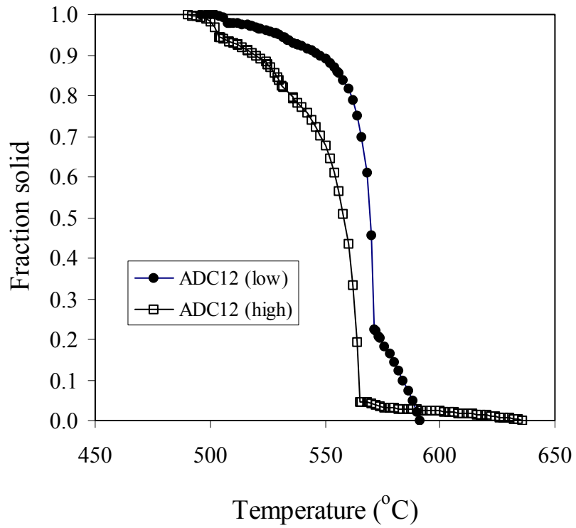
Figure 4. Calculated fraction solid vs. temperature plots of two ADC12 Al-alloys.
