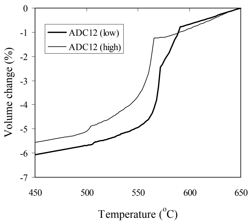
Figure 5. Calculated volume change vs. temperature plots of two ADC12 Al-alloys.
