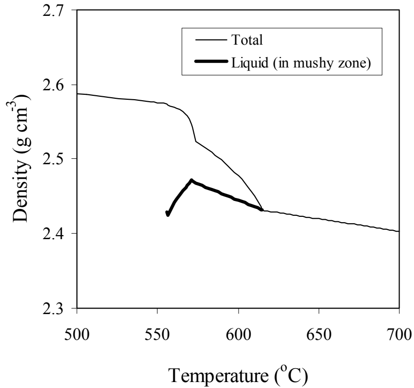
Figure 6. Calculated density of a 356 Al-alloy (with low Cu, Mn and Zn) during solidification. Bold line shows density of the liquid in the mushy zone
