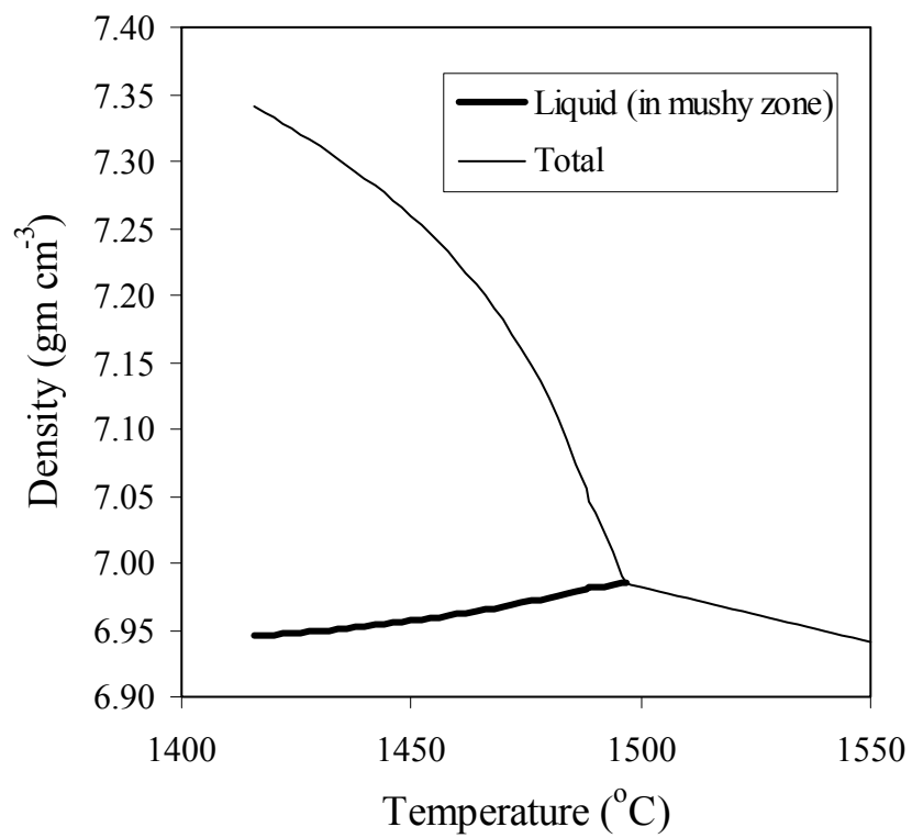
Figure 11. Calculated density of a ZMC711 Mg-alloy during solidification. Bold line shows density of the liquid in the mushy zone
