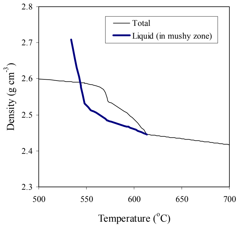
Figure 7. Calculated density of a 356 Al-alloy (with high Cu, Mn and Zn) during solidification. Bold line shows density of the liquid in the mushy zone
