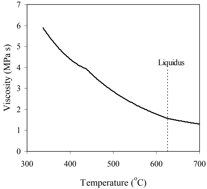
Figure 10. Calculated viscosity of a ZMC711 Mg-alloy during solidification.
