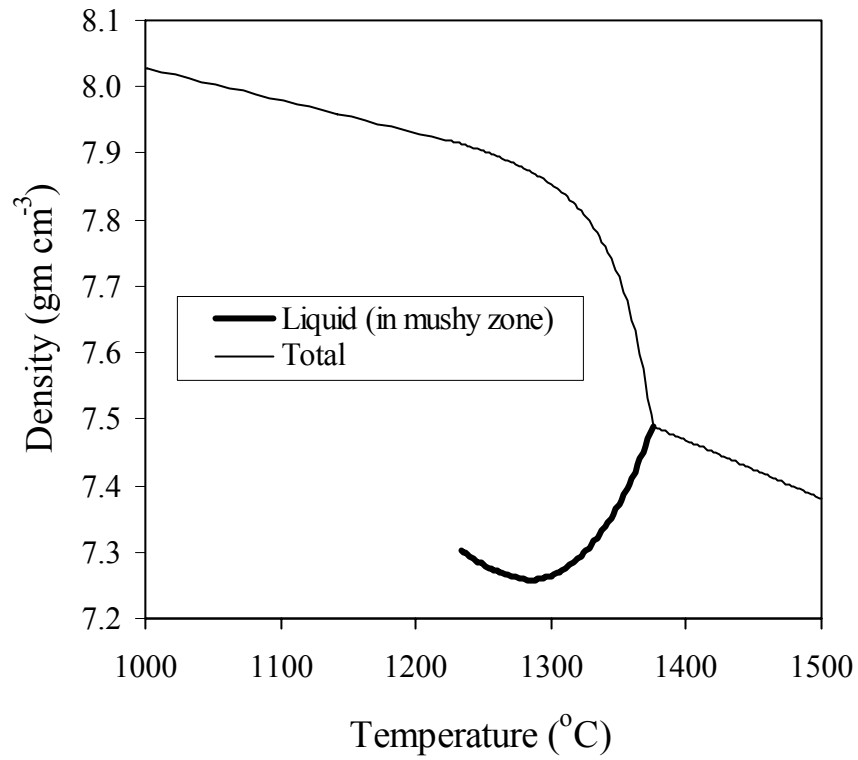
Figure 8. Calculated density of a SRR99 single crystal superalloy during solidification [18]. Bold line shows density of the liquid in the mushy zone
